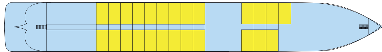
Main deck
